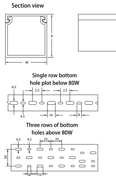
Width 40 and above are all with anti-skid strips, except 45W
