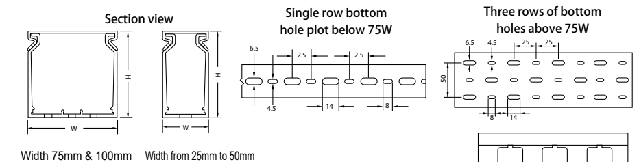
Width 75mm & 100mm Width from 25mm to 50mm
