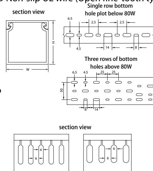
N-VD Non-slip UL wire (Open fine-tooth type)
