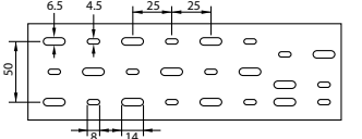
Three rows of bottom holes above 80W
