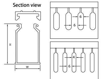
L-VD low smoke halogen-free wiring duct (open fine-tooth type)
