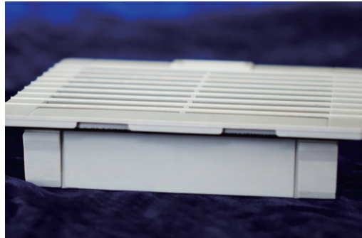
Patented design of the drainage holes in the bottom,ensure IP55
